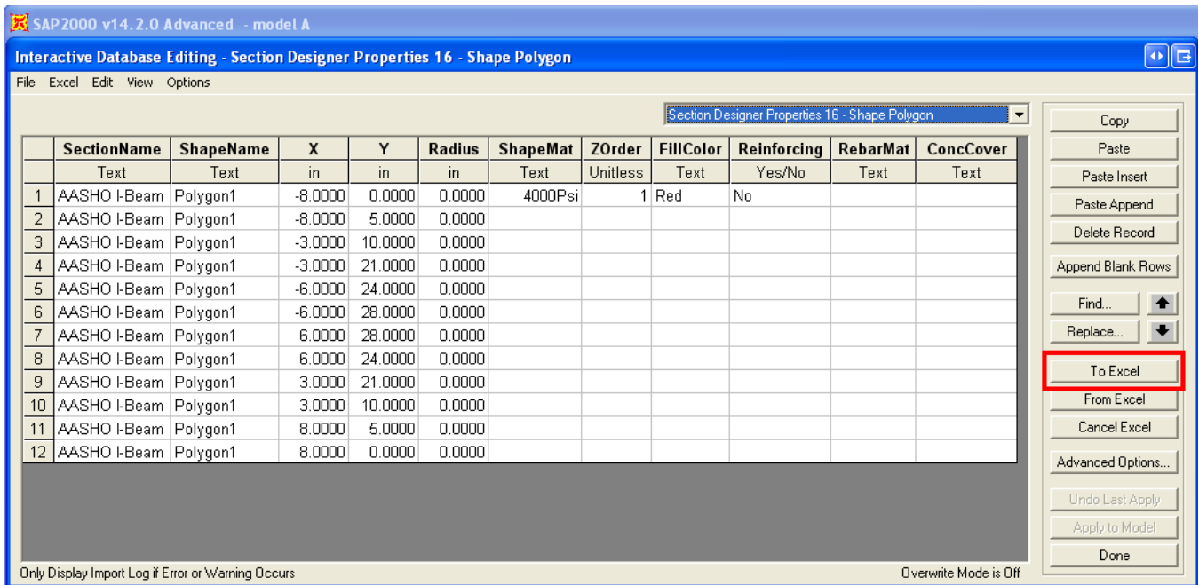
Figure 6 - To Excel
