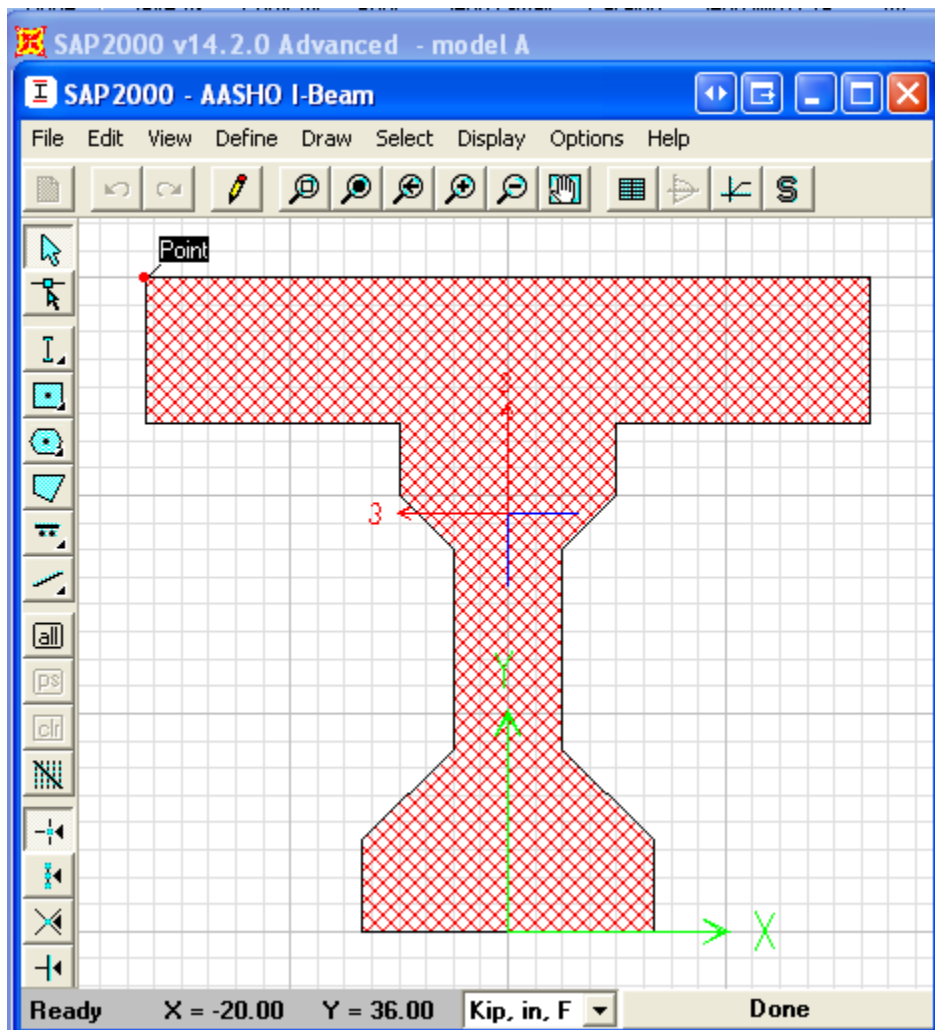
Figure 8 - Final section
