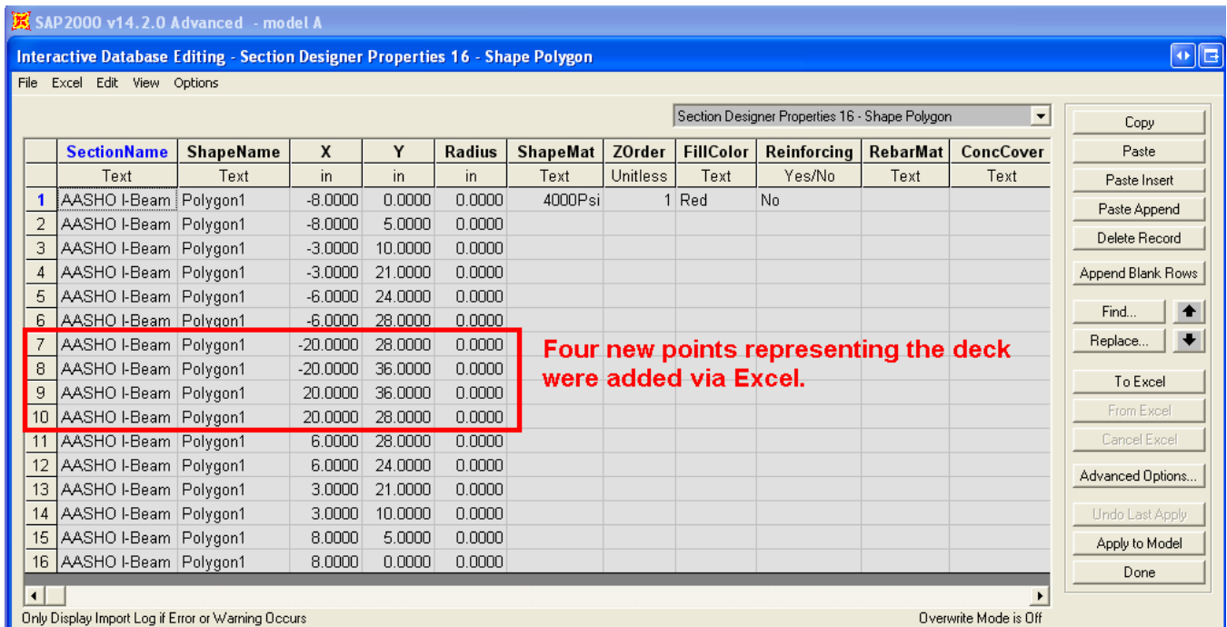
Figure 7 - From Excel
