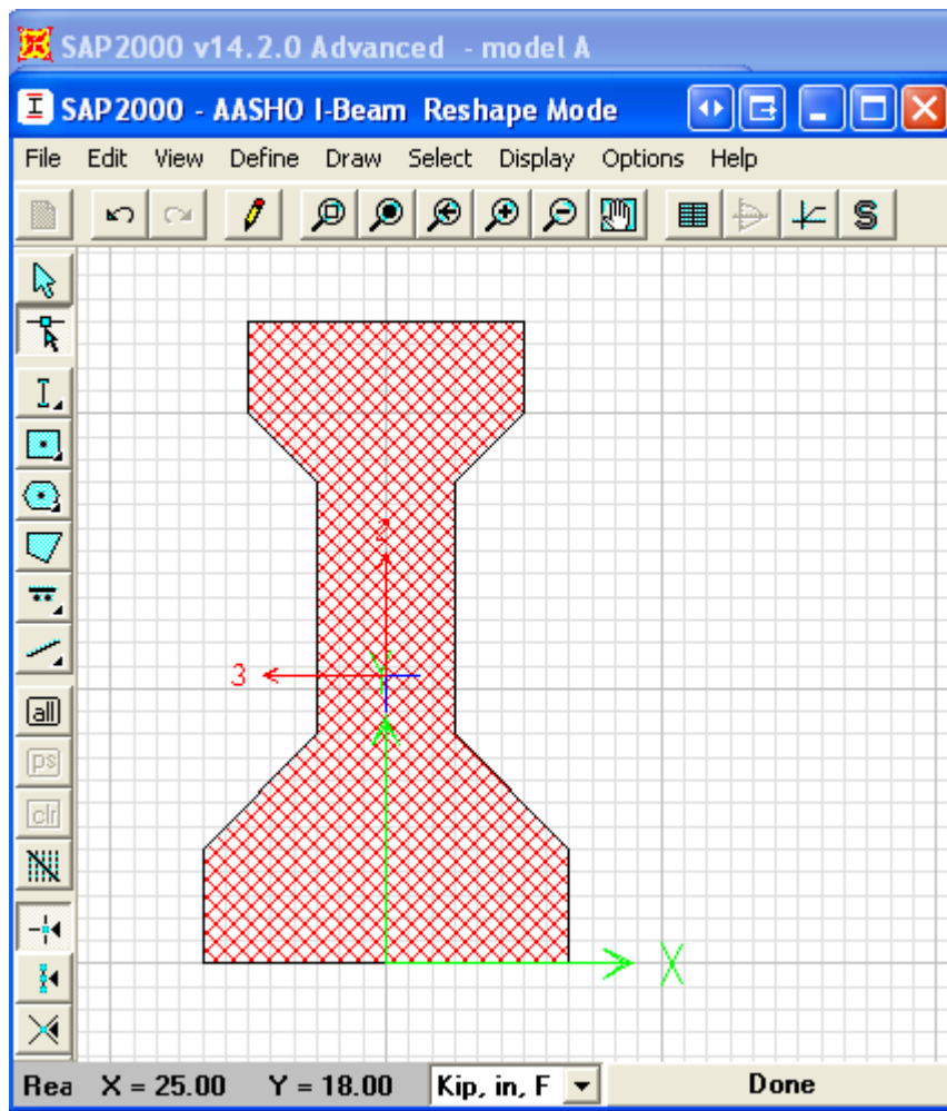
Figure 3 - Section drawn
