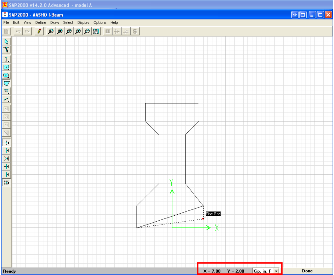
Figure 2 - Draw section
