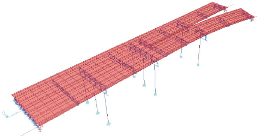
Figure 1 - SAP2000 Bridge Examples model
