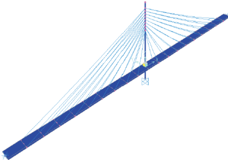
Figure 1 - SAP2000 Bridge Examples model
