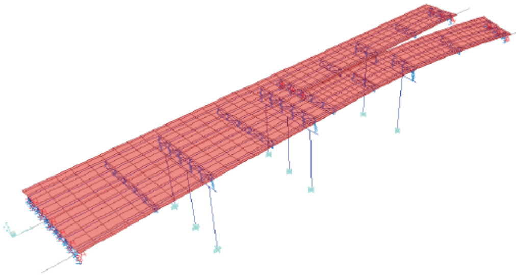
Figure 1 - SAP2000 Bridge Examples model
